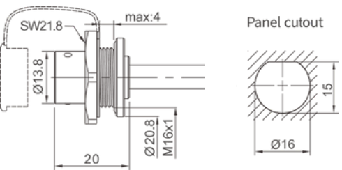
Front-nut mount MatewithSF1220,SF1224
